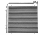
Model:PC200-7Hydraulic Oil Cooler Size:955*750
