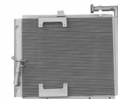
Model:R215-7 Hydraulic Oil Cooler Size:1020*740
