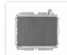
Model: DH225-7 Hydraulic Oil Cooler Size: 840*982
